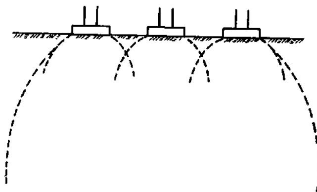
Fig. 4.11 Overlapping of pressure bulbs.
