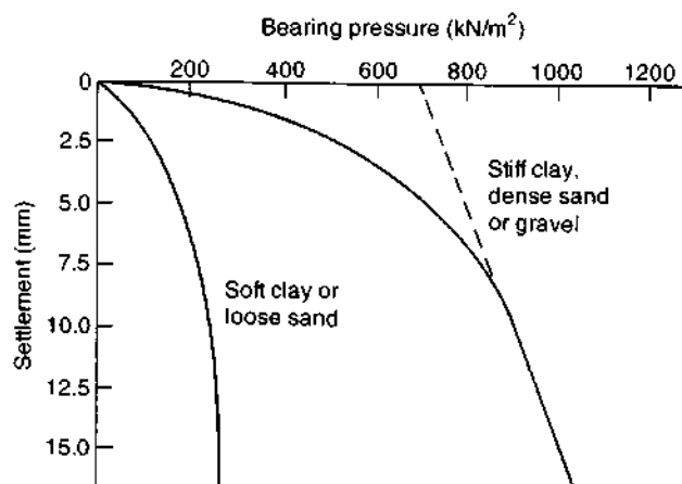
Fig. 8.11 Typical plate loading test results.
