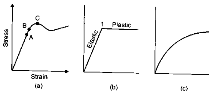
Fig. 4.1 Stress-strain relationships.
