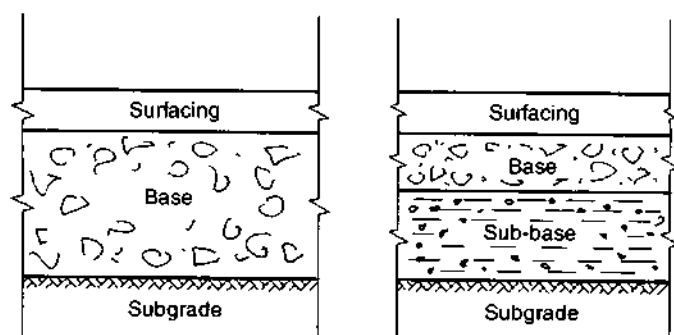
Fig. 11.9 Pavement construction.
