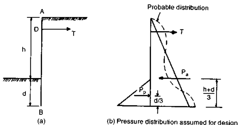
Fig. 7.12 Free earth support method for anchored sheet pile walls.
