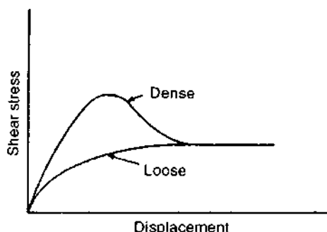
Fig. 3.41 Stress–displacement characteristics of sands.
