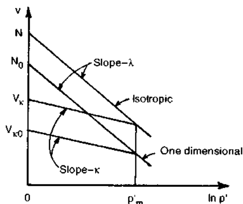
Fig. 13.3 Isotropic and one-dimensional consolidation.
