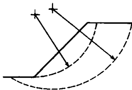
Fig. 5.5 Example of two possible slip surfaces.
