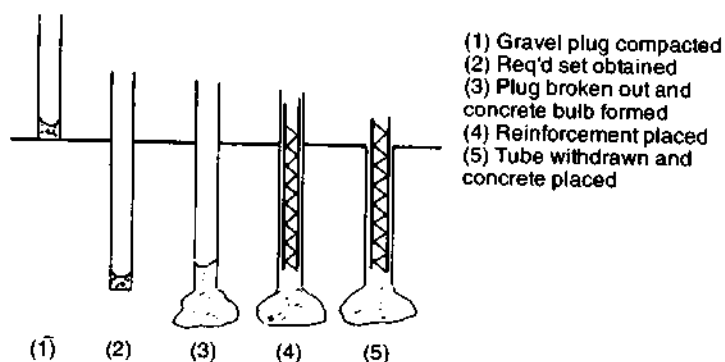
Fig. 8.19 Installation of a Franki pile.
